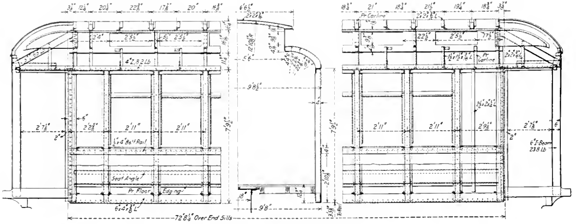
Side Framing of the D. & H. Coaches
